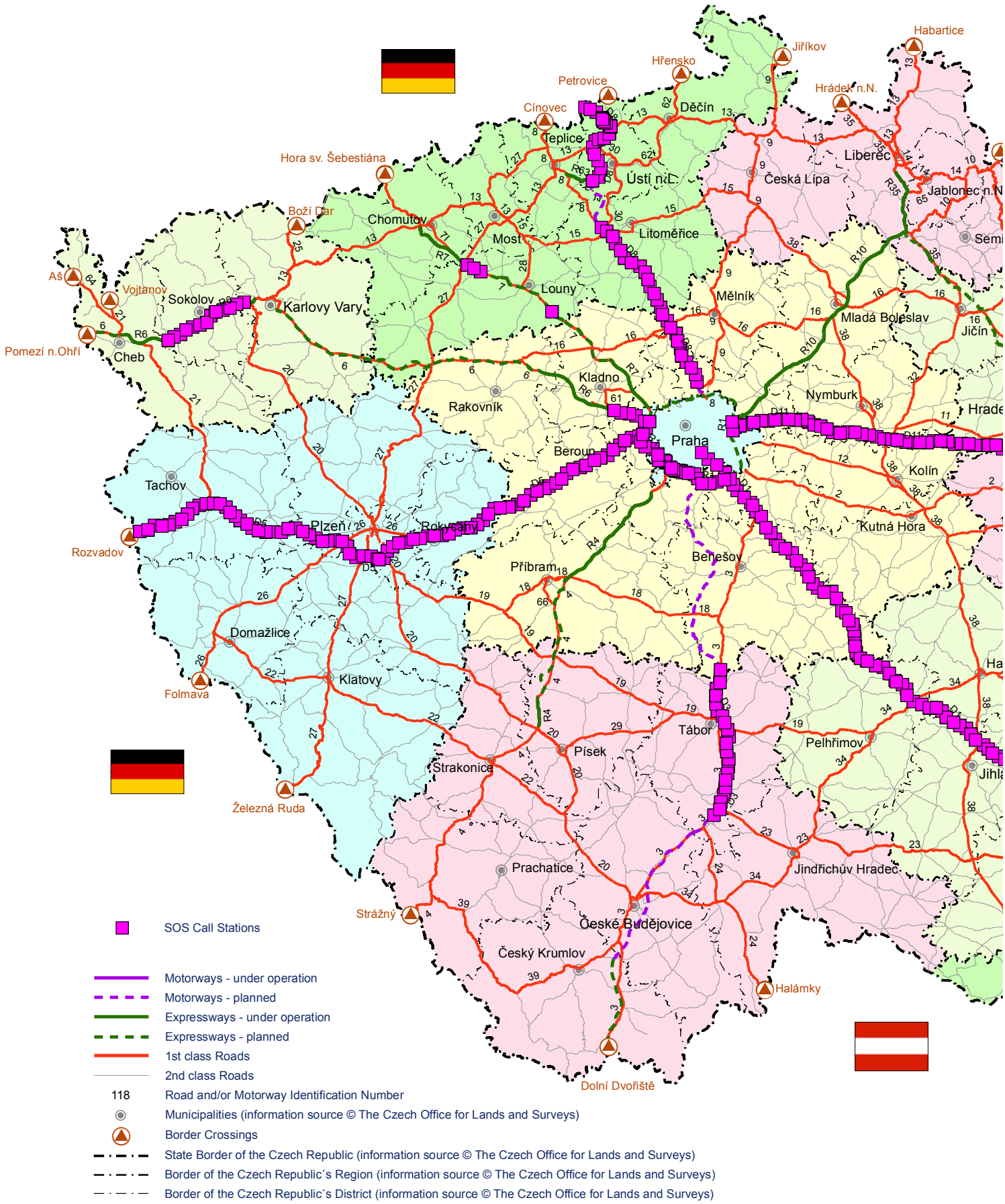
Map No. 9: Emergency call stations (map; photo: source ŘSD)
