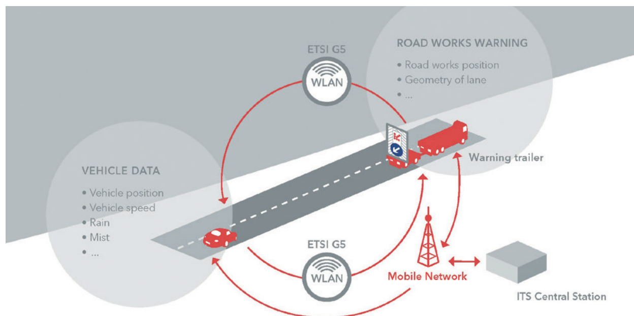
Figure: Interconnection of individual elements (source: www.c-its-korridor.de )
