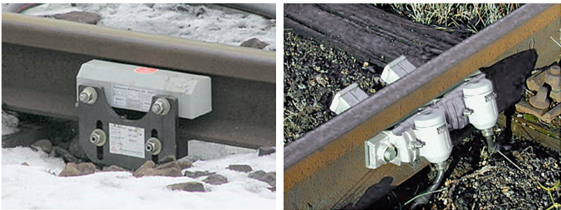
Picture: Axle counters (Photo: SŽDC)
