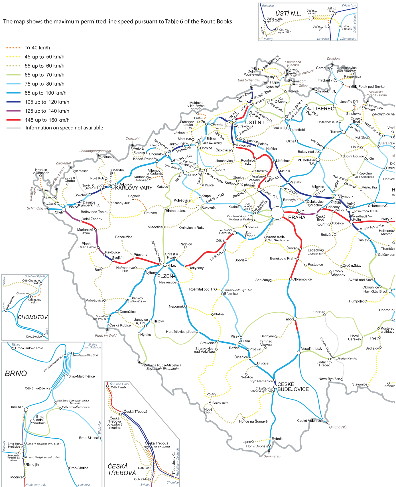
Map No. 11: Maximum permitted line speed (map: source SŽDC)
